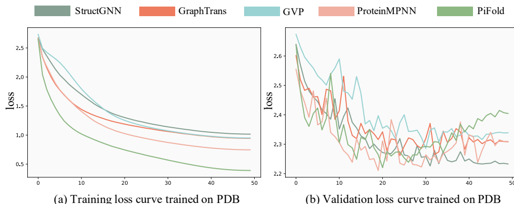
Figure 7: Training and validation loss curves for inverse folding models on Debiased AFDB.
