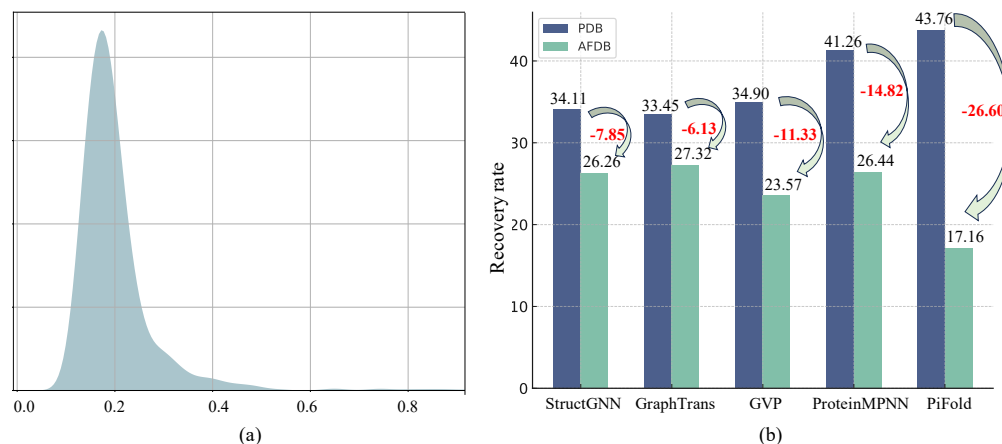
Figure 1: (a) The RMSD distribution of paired structure data from AFDB and PDB. (b) Recovery rate of representative inverse folding methods trained on PDB and AFDB.
