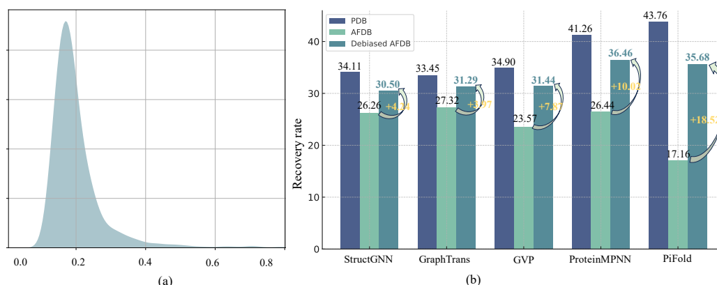
Figure 6: (a) The RMSD distribution of paired structure data from Debiased AFDB and PDB. (b) Recovery rate of inverse folding methods trained on three datasets and evaluated on CATH 4.2.
