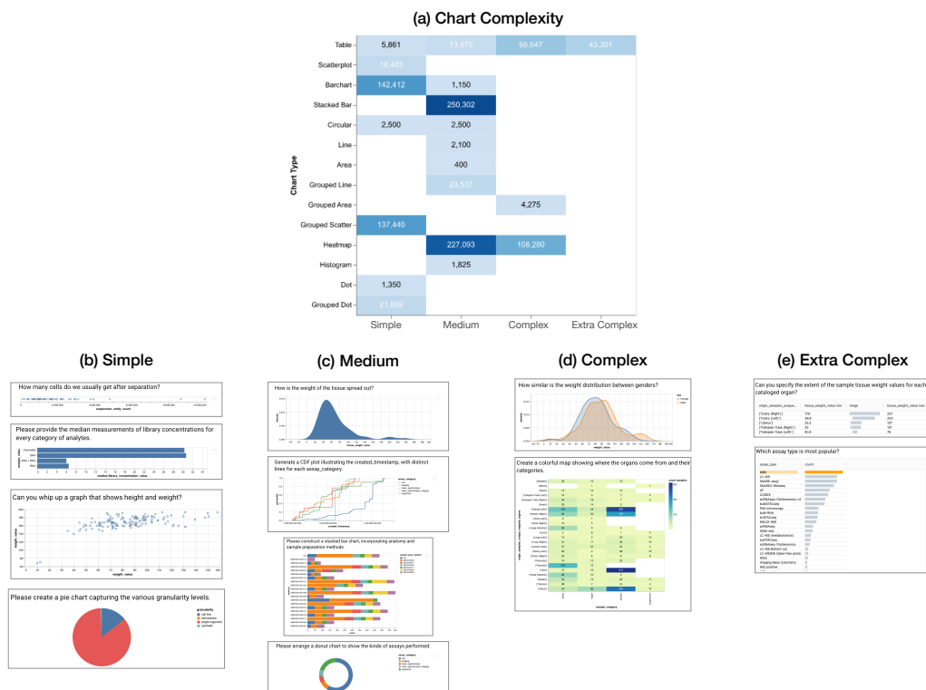
Figure 2: (a) DQVis contains 14 chart types with varying degrees of complexity. Complexity is determined by the number of keys in the visualization specification. (b) Simple visualizations have \leq 12 keys; (c) Medium \leq 24 ; (d) Complex \leq 36 ; and (e) Extra Complex is > 36 .
