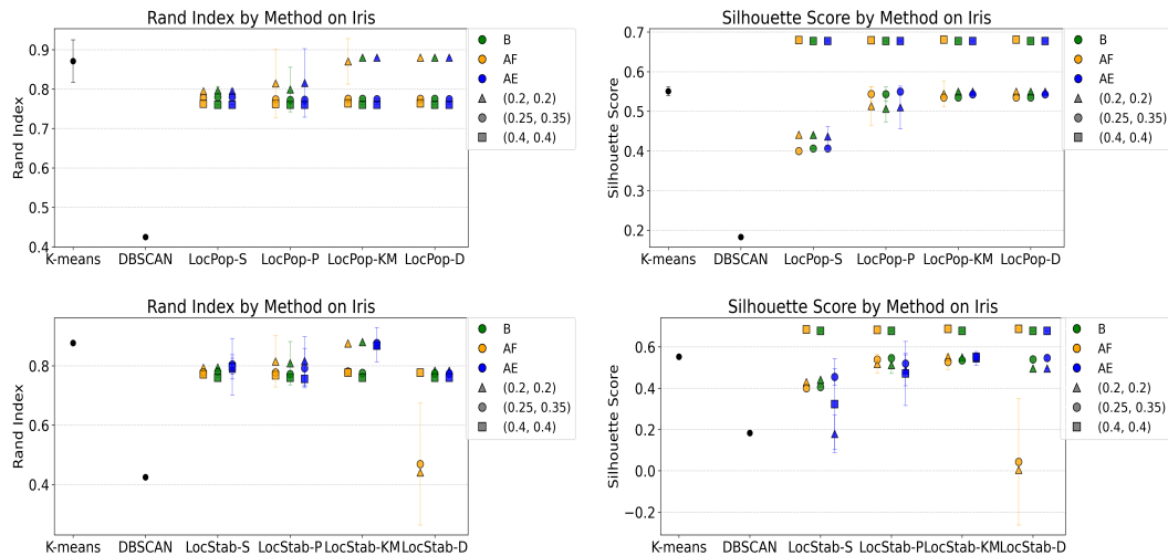
Figure 9: Comparing Rand index (left) and silhouette score (right) of k -means, DBSCAN and LocPop (top) or LocStab (bottom) variants for the Iris dataset.
