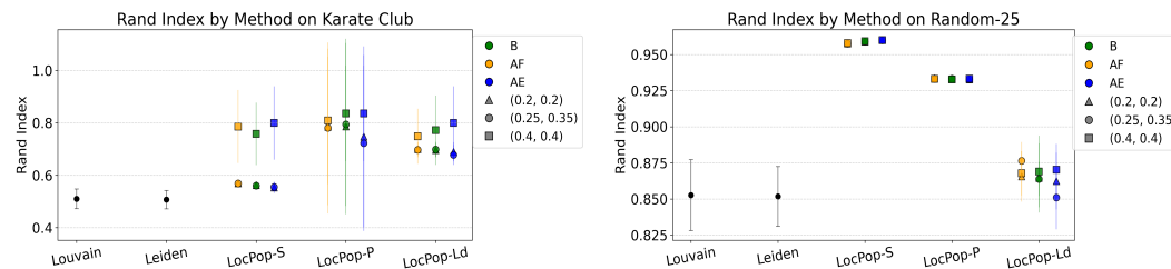
Figure 3: Comparing Rand index of Leiden, Louvain, and LocPop variants on the Karate club dataset (left) and the synthetic dataset Random-25 (right). In all figures henceforth, 2-sigma error bars show the standard deviation of the plotted data.
