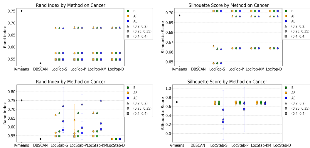
Figure 10: Comparing Rand index (left) and silhouette score (right) of k -means, DBSCAN and LocPop (top) or LocStab (bottom) variants for the Cancer dataset.
