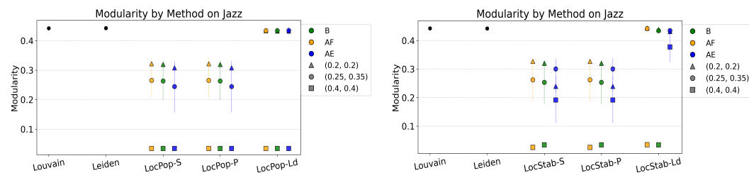
Figure 6: Comparing modularity of Louvain, Leiden, and LocPop (left) or LocStab (right) variants for the Jazz dataset.
