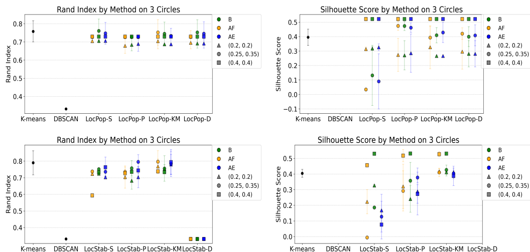
Figure 12: Comparing Rand index (left) and silhouette score (right) of k -means, DBSCAN and LocPop (top) or LocStab (bottom) variants for the 3 Circles dataset.
