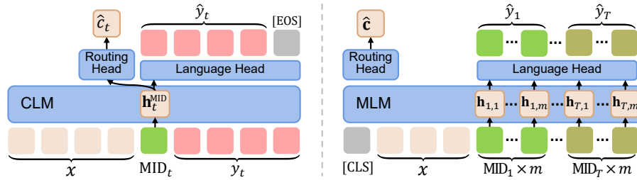
Figure 3: Architectures for response-aware routing in Lookahead . Left : Sequence-level modeling with a causal language model (CLM), where the hidden state at the MID token encodes the response information. Right : Token-level modeling with a masked language model (MLM), where fully masked responses are reconstructed and summarized via attention over MID tokens.
