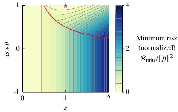
Figure 3: Concept shift induces a phase transition in generalization behavior. We depict minimum prediction risk \mathcal{R}_{\min} of optimally tuned ridge regression ( \lambda = \gamma / \text{SNR} ) as \kappa and \cos \theta vary, see Eq (10) for definitions. No concept shift corresponds to \kappa = \cos \theta = 1 (star). The thick curve, \kappa \cos \theta = 1/2 , separates the weak and strong concept shift regimes. More training data improves generalization only when concept shift is weak, \kappa \cos \theta > 1/2 . Outside this region, any data hurts generalization.
