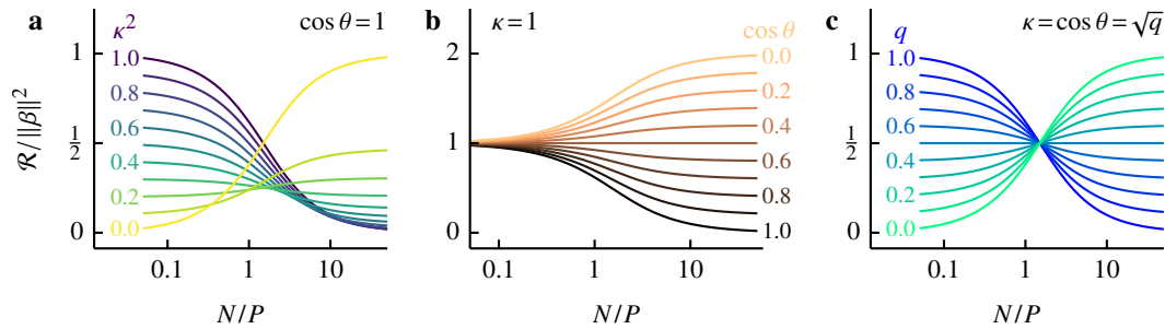
Figure 2: More data hurts performance when concept shift is strong. We depict the data dependence of asymptotic prediction risk for isotropic features, Eq (9), under three concept shift settings of varying degree, parametrized by coefficient alignment \cos \theta = \beta \cdot \tilde{\beta} / \|\beta\| \|\tilde{\beta}\| and scaling factor \kappa = \|\tilde{\beta}\| / \|\beta\| (see legend). a Shrinking coefficients : \tilde{\beta} = \kappa \beta . b Rotating coefficients : \|\tilde{\beta}\| = \|\beta\| but \theta varies. c Mixture of robust and nonrobust features : \tilde{\beta}_i = \beta_i if feature i is robust, otherwise \tilde{\beta}_i = 0 . This setting is parametrized by q = \kappa^2 = \cos^2 \theta . We set \text{SNR} = 1 in a-c, and the regularization is in-distribution optimal \lambda = \gamma / \text{SNR} .
