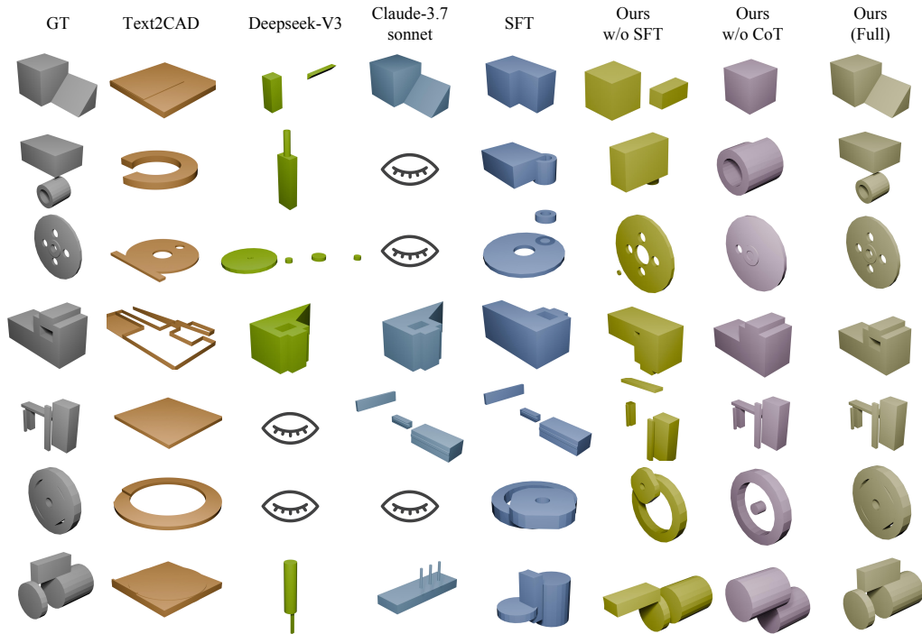
Figure 3: Qualitative comparison between baseline methods and different model variants under various training strategies. Text2CAD is a command-sequence-based baseline; Deepseek-V3 and Claude-3.7 represent open-source and proprietary LLMs, respectively. The right columns show our ablations and full model, which best preserve structure and geometry.
