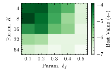
Figure 10: Ablation for on unconstrained out-of-model functions.
