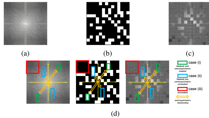
Figure A: Failure in spectral information extraction with the original MAE pre-training. (a) Input spectrum magnitude. (b) Patch embedding mask for inference. (c) Poor-quality reconstruction from (a) and (b). (d) Explanation of reconstructed patches in (c).
