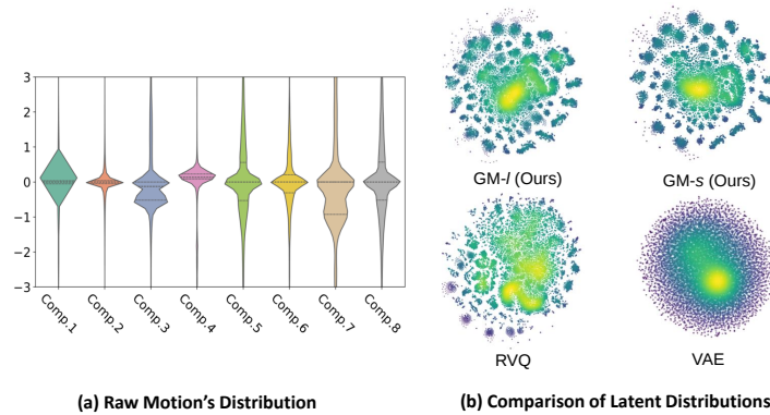
Figure 1: (a) Violin map of the motion's moving components randomly selected from the normalized HumanML3D datasets;(b) Visualization of different representation model's latent space with t-SNE. Yellow indicates dense sample distribution, while blue represents sparse sample distribution.
