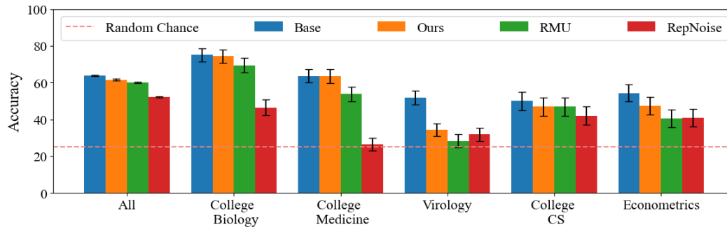
Figure 2: When erasing WMDP concepts, we expect accuracy to remain high for unrelated (safe) MMLU concepts. ELM shows stronger specificity, with less of a decrease in accuracy after fine-tuning Zephyr-7B.
