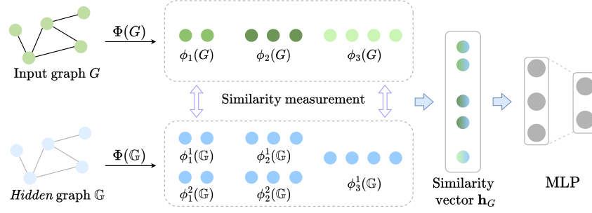
Figure 2: An overview of HSP-GKN. \Phi(\cdot) is the hierarchical graph feature mapping.
