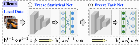
Figure 2: Two-stage training procedure for HStat-Net.
