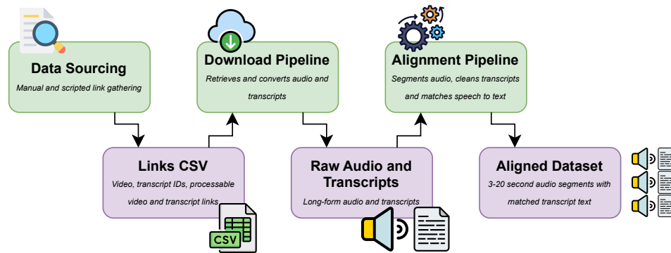
Figure 1: Overview of the EUROSPEECH data processing pipeline. The workflow begins with the initial Data Sourcing and Metadata Collection phase, which gathers metadata from parliamentary websites and APIs. This structured information (as Links CSV ) feeds into the Download Pipeline to retrieve raw audio and transcripts. The Raw Audio and Transcripts are then processed by the Alignment Pipeline , which segments the audio and matches it to the corresponding text. The final output is the Aligned Dataset , consisting of short audio segments paired with their transcriptions, ready for model training.
