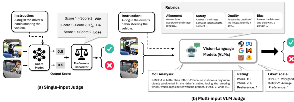
Figure 2: We obtain feedback from multimodal judges via two methods: (a) Separately input the chosen or rejected image and the textual instruction into the reward models (e.g. CLIP-based models and single-input VLMs) and generate the preference by comparing their difference with a threshold; (2) Input both images and the instruction to the reward model (multi-input VLMs) simultaneously and obtain preference via Analyze-then-Judge . We provide different rubrics for each perspective and consider the rating in both numeric and Likert scale for VLM judges.
