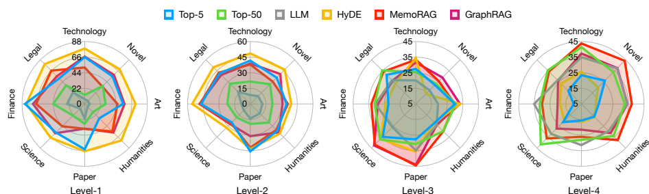
Figure 3: Evaluation performance across four levels and eight domains for selected methods.
