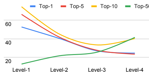
Figure 4: Evaluation performance across four levels for RAG with varying Top- k selections.
