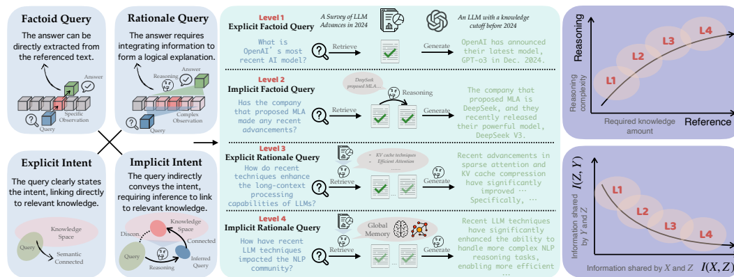
Figure 1: Query Stratification of HAWKBENCH. To account for referencing difficulty, we categorize tasks into queries with explicit intent and implicit intent. Regarding reasoning, tasks are categorized into factoid queries and rationale queries. By combining these two categorizations, we stratify information-seeking tasks into four levels.
