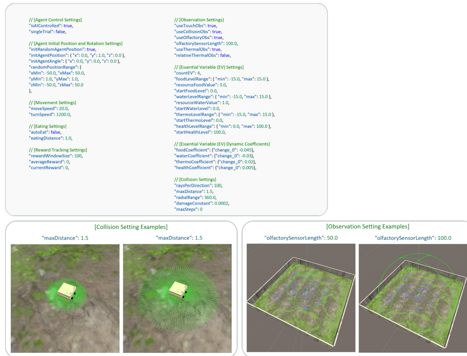
Figure 10: Agent configuration parameters in EVA. Top: JSON snippets illustrating control, movement, eating, essential variable (EV) decay, observation, and collision settings. Bottom: Visualization of selected parameters, including collision sensing range (maxDistance) and olfactory sensor range (olfactorySensorLength). These settings govern how agents perceive the environment and manage internal state variables.
