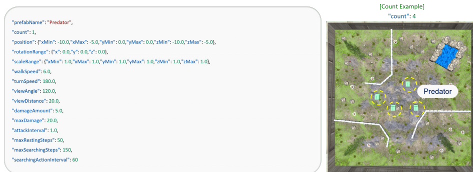
Figure 16: Predator deployment configuration in EVA. Left: JSON configuration for a predator agent, including key parameters such as position range, view angle (120 degrees), walk speed, and state transition limits (e.g., ‘maxRestingSteps’, ‘maxSearchingSteps’). Right: Visualization of four predators navigating using Unity’s NavMesh system.
