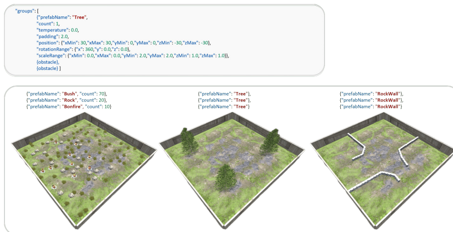
Figure 14: Obstacle configuration in EVAAA. Top: JSON configuration specifying parameters for static obstacles such as trees, including position, padding, and scale. Bottom left: Randomized placement of bushes, rocks, and bonfires to create unorganized terrain. Bottom center: Organized (or structured) placement of tree obstacles with consistent spacing. Bottom right: Placement of walls to obstruct navigation or visual perception.
