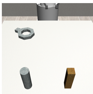
RoboSuite - Round
