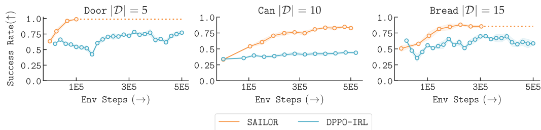
Figure 6: We find that SAILOR is significantly more interaction-efficient than a model-free inverse RL baseline that directly updates DP policy parameters via DPPO [Ren et al., 2024a].
