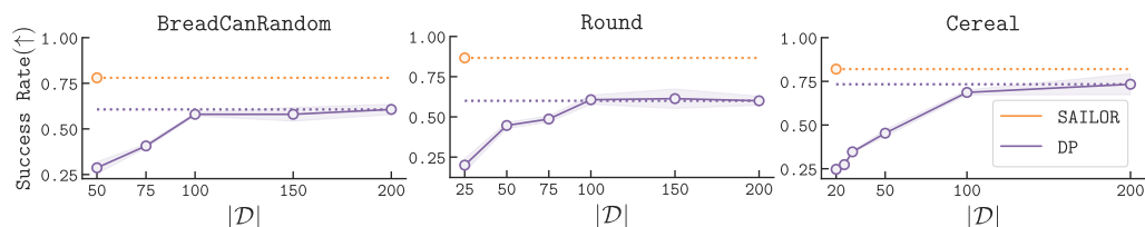
Figure 5: We see that simply scaling up the amount of demos |\mathcal{D}| used for training DP via behavioral cloning by 5-10 \times often plateaus in performance and is unable to match the performance of SAILOR.
