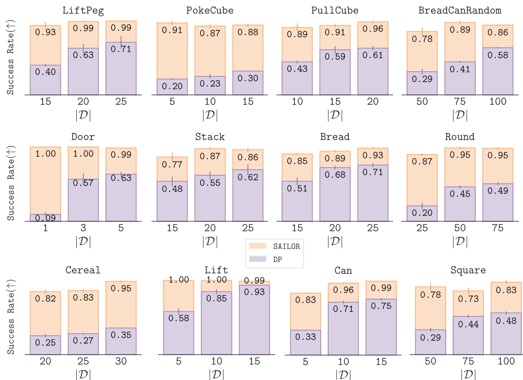
Figure 4: Across 12 visual manipulation problems from 3 benchmarks, SAILOR consistently outperforms diffusion policy (DP) trained on the same demos, where |\mathcal{D}| denotes the number of demos.
