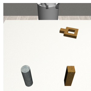
RoboMimic - Square
