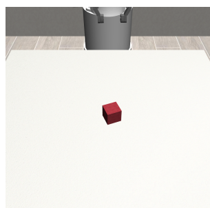
RoboMimic - Lift
