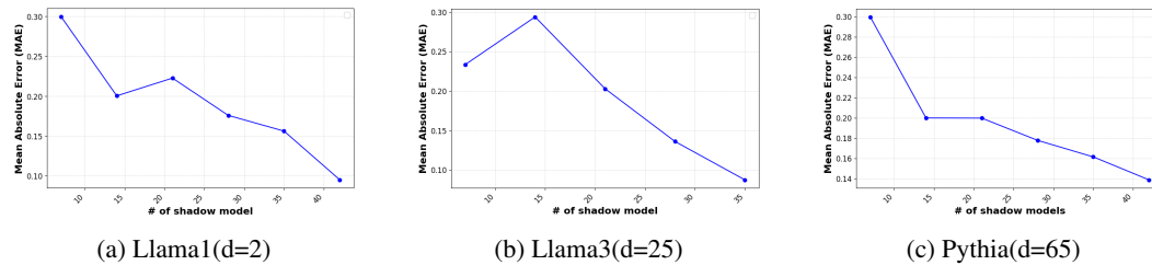
Figure 5: Effect of number of shadow models k_1 \cdot k_2 in Q&A mode and gender property. The y axis is the Mean Absolute Errors across different target ratios.
