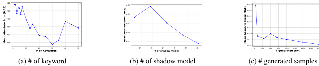
Figure 2: Effects of hyperparameters of our attacks for Llama-3 and gender property.
