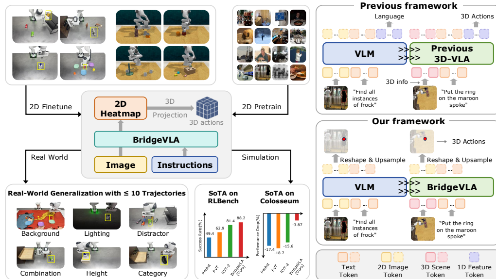
Figure 1: Overview. BridgeVLA is a novel 3D VLA model that aligns the input and output within a unified 2D image space. It is pre-trained on object grounding using 2D heatmaps and fine-tuned on action prediction for 3D manipulation. Experiment results in both simulation and the real world show that it is able to learn 3D manipulation both efficiently and effectively.
