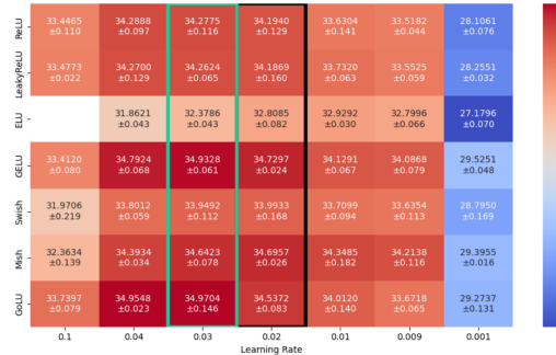
Figure 13: Test Mask mAP - Mask R-CNN-PFN ResNet-50 on MS-COCO. The default learning rate is 0.02 which is colored in black and the best learning rate is 0.03 which is colored in green.
