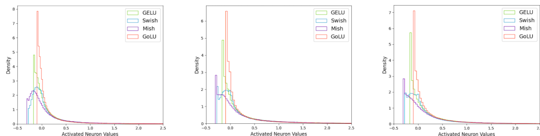
Figure 4: Distributions of final activation outputs of ResNet-50 trained on ImageNet-1k for three randomly sampled images from ImageNet-1k. GoLU leads to a more peaked distribution for the final activation output.
