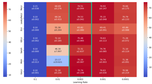
Figure 15: Test accuracies - ViT-B/32 on ImageNet-1k. The default learning rate is 0.003 which is also the best and is colored in green.
