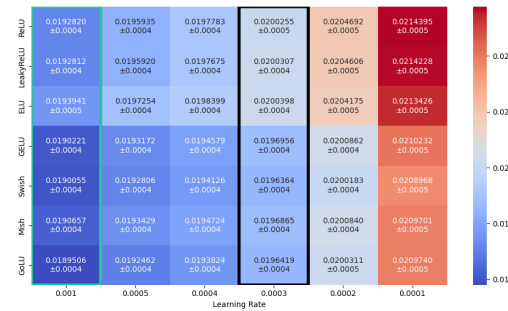
Figure 11: Test Loss - DDPM on CelebA. The default learning rate is 0.0003 which is colored in black and the best learning rate is 0.001 which is colored in green.
