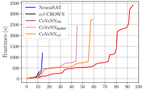
(a) Solved problems sorted by runtime.
