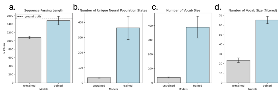
Figure 12: Comparison between trained and untrained RNNs on sequences with overlapping words across 10 independent runs and randomly initialized RNNs. a. Sequence parse length. Dashed line is the ground truth sequence parsing length. b. Number of unique neural population states. c. Chunk dictionary size. d. Chunk dictionary size (filtered desolate chunks (threshold=5)) Error bars represent the standard error of the mean.
