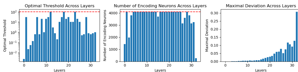
Figure 16: Layer-wise statistics of PA extracted chunks commonly proceeding the concept “of”.
