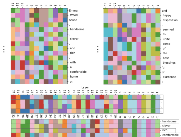
Figure 7: Upper: Describing the network’s processing of tokens as the succession of unsupervised learned chunks. Lower: Layer-wise processing of similar token types.
