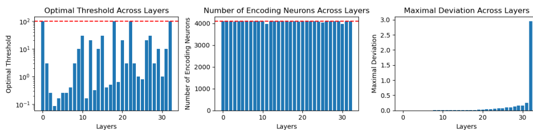
Figure 17: Layer-wise statistics of PA extracted chunks encoding the latest word being “people”.
