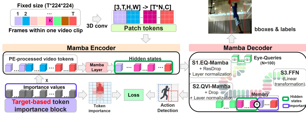
Figure 2: Overview of the proposed structure. The encoder processes PE-embedded video tokens through Mamba layers, accompanied by a target-based token importance block that highlights informative regions for action detection. The decoder then operates on two Mamba-based modules followed by a linear layer. Illustration corresponds to batch size = 1. (EQ-Mamba: Eye Query-based Mamba, QVI-Mamba: Query-Video Information-fused Mamba, PE: Positional Embedding, ResDrop: Residual connection with Dropout, Drop: Dropout, K: Key frame.)
