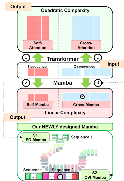
Figure 1: Motivation of MOGO. Comparison between Transformer and Mamba complexity inspires our framework design. By Mamba-izing the Transformer's (1) attention architecture, our framework enables (2) linear transformation for single-sequence modeling and (3) selective copying mechanism for cross-sequence modeling.
