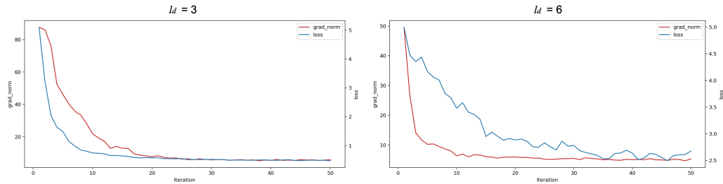
Figure S1: Training curves and diagnostics. Training loss (right axis) and gradient norm (left axis) for decoder depths l_d > 1 .
