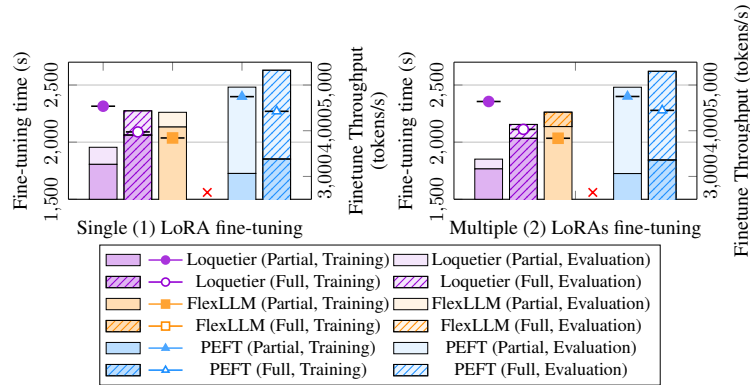
Figure 3: Comparison of the performance of Loquetier, FlexLLM and PEFT in fine-tuning tasks. The meanings of Partial and Full are the same as in Figure 2. × indicates that the results were not obtained: FlexLLM does not support backward propagation computations for modules other than up, gate and down. PEFT can only finetune one LoRA adapter at a time, so its time cost is cumulative.
