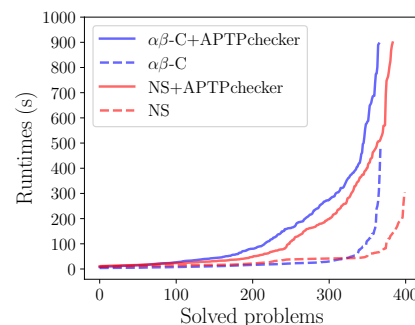
Fig. 3: Runtimes and problems solved.
