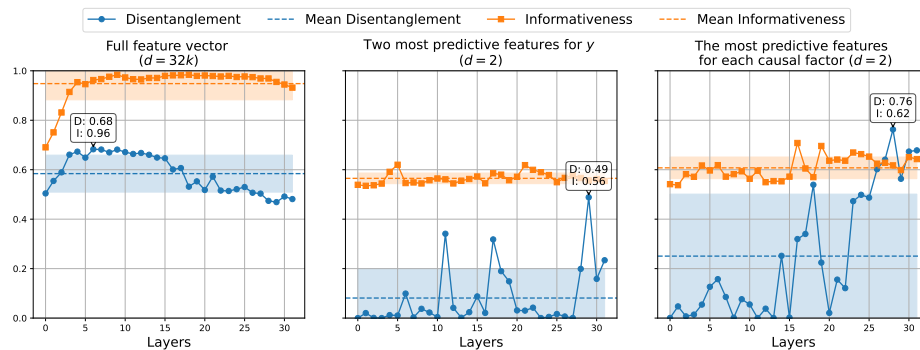
Figure 3: Disentanglement and informativeness scores for 32k-dimensional SAEs across model layers. Solid lines indicate layer-wise scores, dashed lines denote the mean, and shaded regions represent \pm 1 standard deviation. Each subplot is annotated with the maximum disentanglement score along with its corresponding informativeness score.
