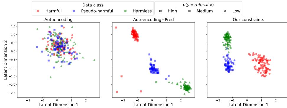
Figure 7: Latent space for refusal behavior in the Qwen2-7B model with autoencoding ( left ), autoencoding + prediction ( center ), and our constraints ( right ).
