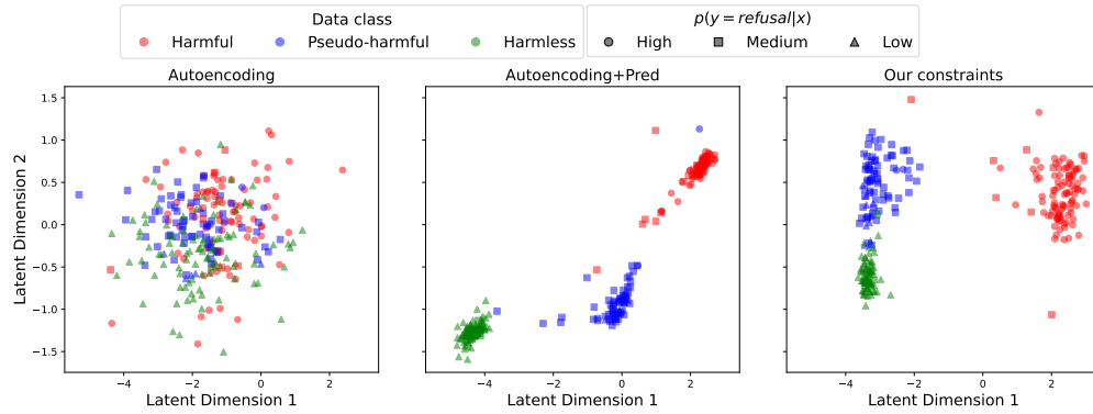
Figure 2: Latent space for refusal behavior in Llama-3.1-8B with autoencoding ( left ), autoencoding + prediction ( center ), and our constraints ( right ). The baseline method entangles the two latent dimensions, but adding the contrastive constraint leads to an aligned latent space.
