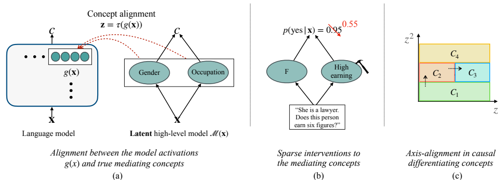
Figure 1: \mathcal{M} represents a high-level model that explains the language model’s behavior c in terms of latent mediating concepts z , such that sparse interventions to mediating concepts suffice to change model behavior. Instead of assuming access to the high-level model \mathcal{M} , our work disentangles the learned representation \hat{z} with the key assumption that causal differentiating concepts are axis-aligned.
