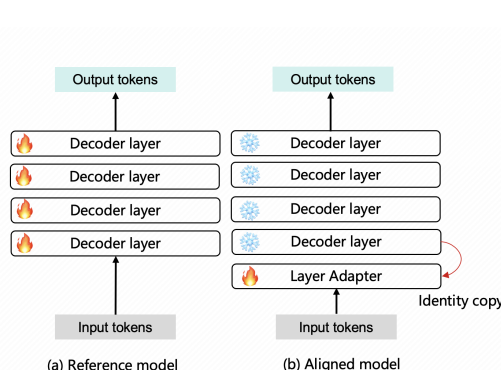
Figure 3: (a) All layers fine-tuning. (b) Fine-tuning on the added identity layer while keeping the original layers of the LM frozen.
