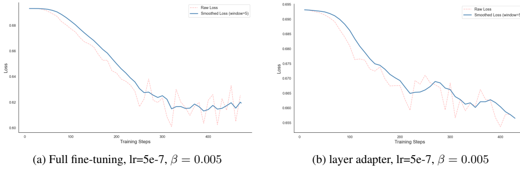
Figure 7: Comparison of two loss curves on Qwen2.5-7B model.
