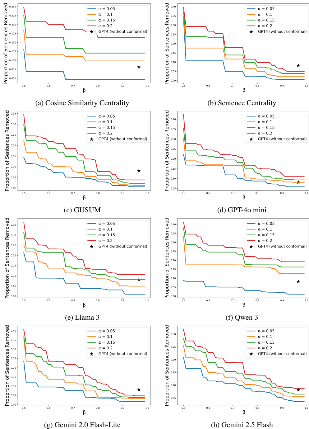
Figure 21: Target recall \beta vs. proportion of sentences removed (conciseness). Lines indicate different values for the target error rate \alpha on MTS.
