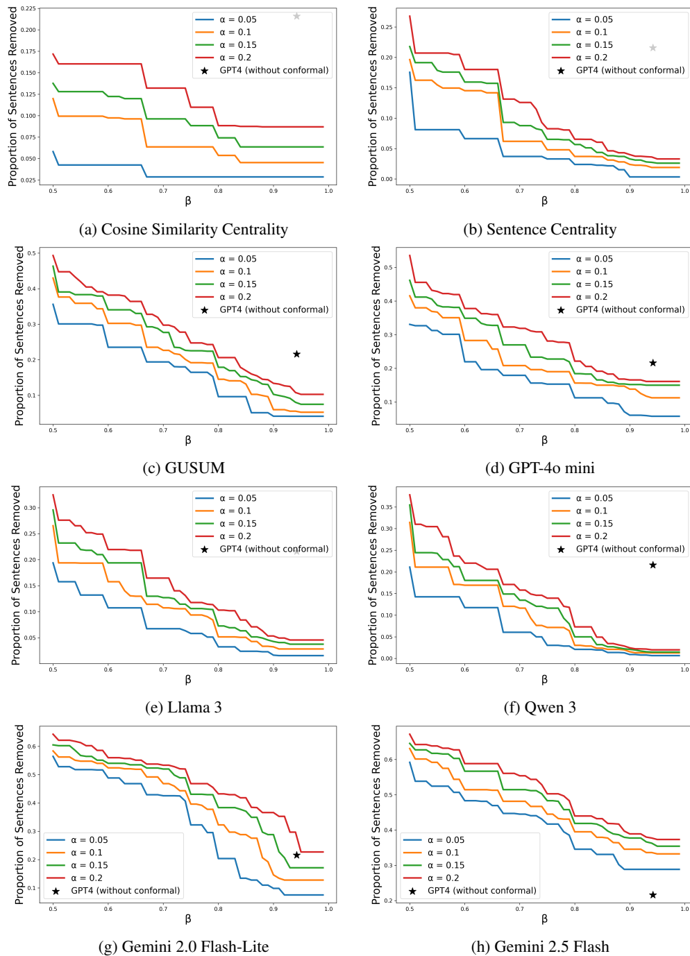
Figure 18: Target recall \beta vs. proportion of sentences removed (conciseness). Lines indicate different values for the target error rate \alpha on CSDS.
