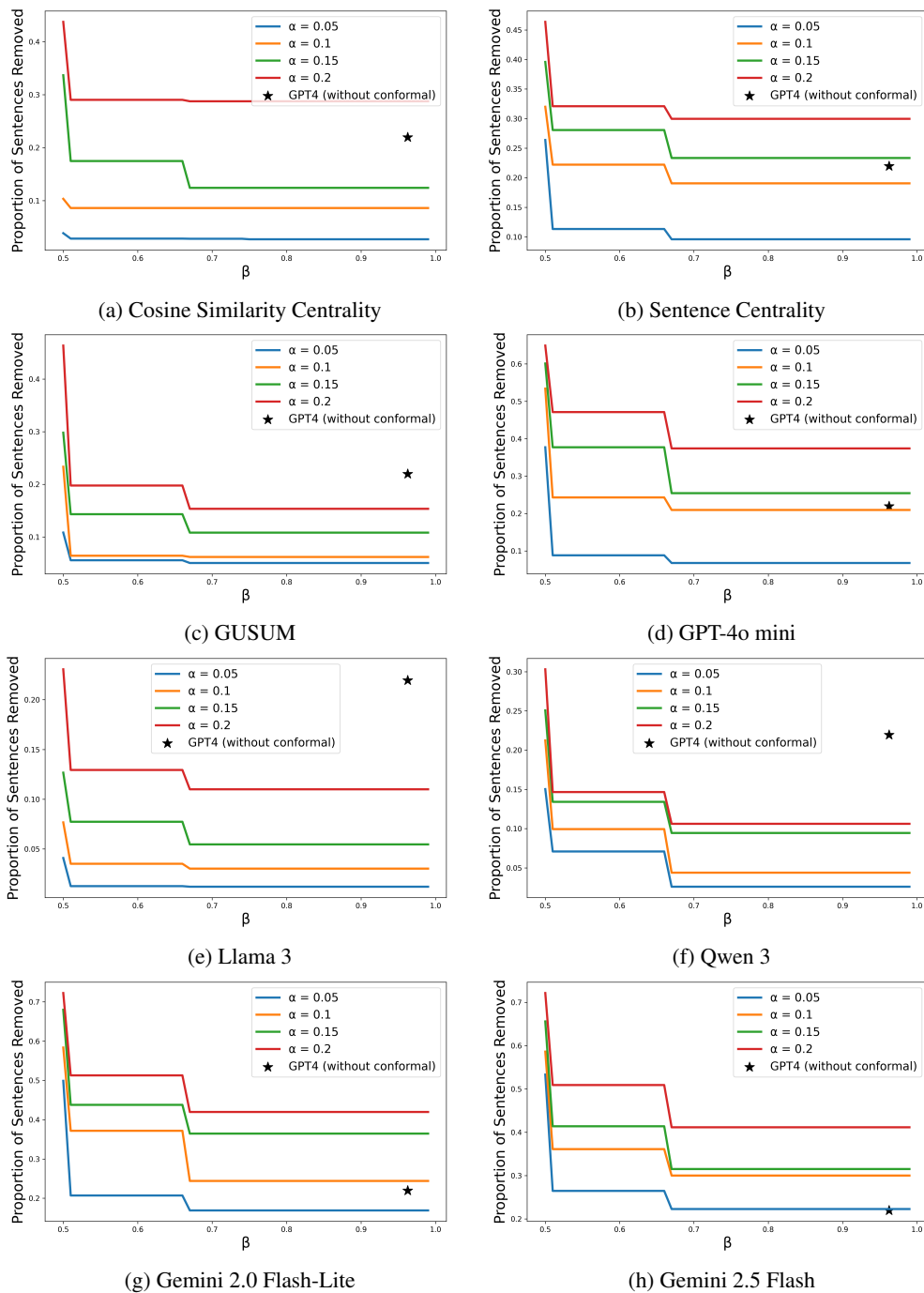
Figure 19: Target recall \beta vs. proportion of sentences removed (conciseness). Lines indicate different values for the target error rate \alpha on TLDR-AIC.
