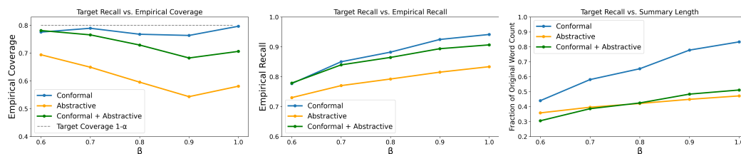
Figure 6: Comparison between extractive summarization with our method, abstractive summarization with an LLM, and our hybrid proposal on ECTSum. Here the target coverage is 1 - \alpha = 0.8 , the conformal approach uses Gemini 2.5 Flash scoring, and the abstractive model is GPT-4o mini.
