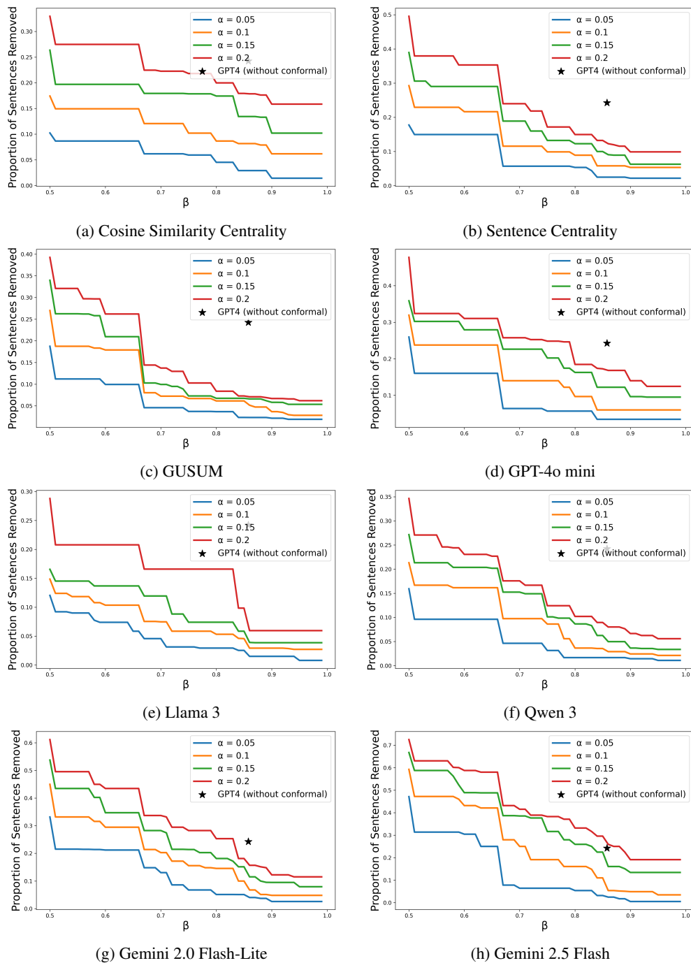
Figure 20: Target recall \beta vs. proportion of sentences removed (conciseness). Lines indicate different values for the target error rate \alpha on ECT.
