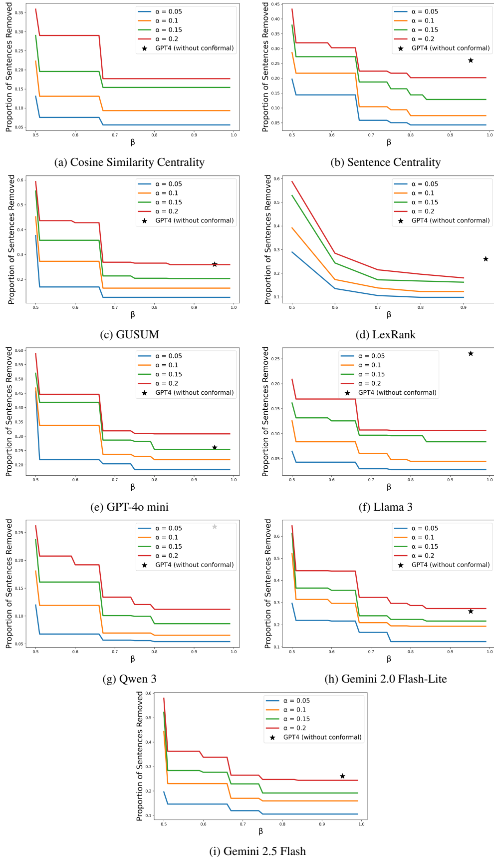
Figure 17: Target recall \beta vs. proportion of sentences removed (conciseness). Lines indicate different
