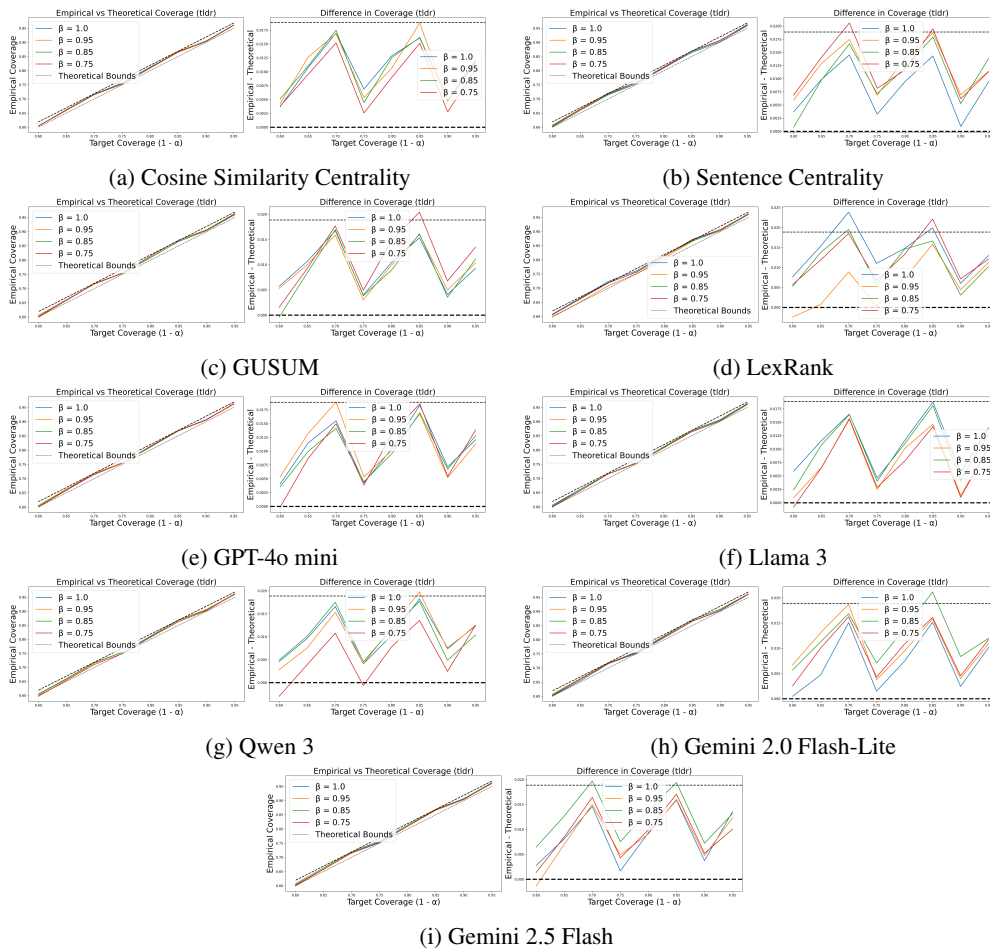
Figure 9: User-specified probability of achieving coverage ( 1-\alpha ) vs. empirical probability of achieving coverage, on the TLDR-AIC dataset. Dashed lines show theoretical bounds given in Theorem 1. Results are averaged over 400 random splits of calibration and test data.
