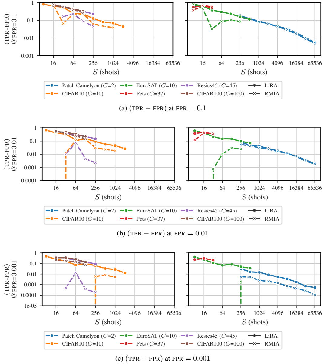
Figure A.7: LiRA and RMIA vulnerability ( (\text{TPR} - \text{FPR}) ) as a function of shots ( S ) when attacking a ViT-B Head fine-tuned without DP on different datasets. For better visibility, we split the datasets into two panels. We observe the power-law for both attacks, but the RMIA is more unstable than LiRA. The lines display the median over six seeds.
