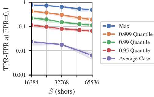
Figure 6: Individual vulnerability for ViT-B (Head) when fine-tuning on Patch Camelyon. We observe a similar power-law relationship for individuals when looking at the quantiles but the max decreases slower. The Average Case shows the average LiRA vulnerability over the individuals also illustrated in the right panel of Figure 3.
