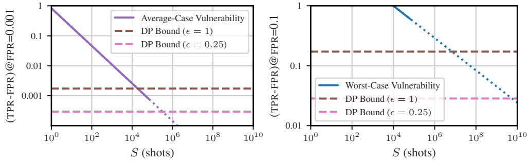
Figure 7: Illustration of the extrapolation for the average-case at FPR = 10^{-3} (left) and worst-case at FPR = 10^{-1} (right).
