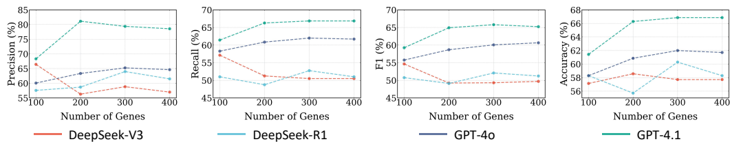
Figure 5: Performance comparison of cell type annotation when scaling context lengths.
