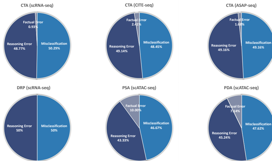
Figure 7: Distribution of DeepSeek-R1's errors within distinct types across various tasks.
