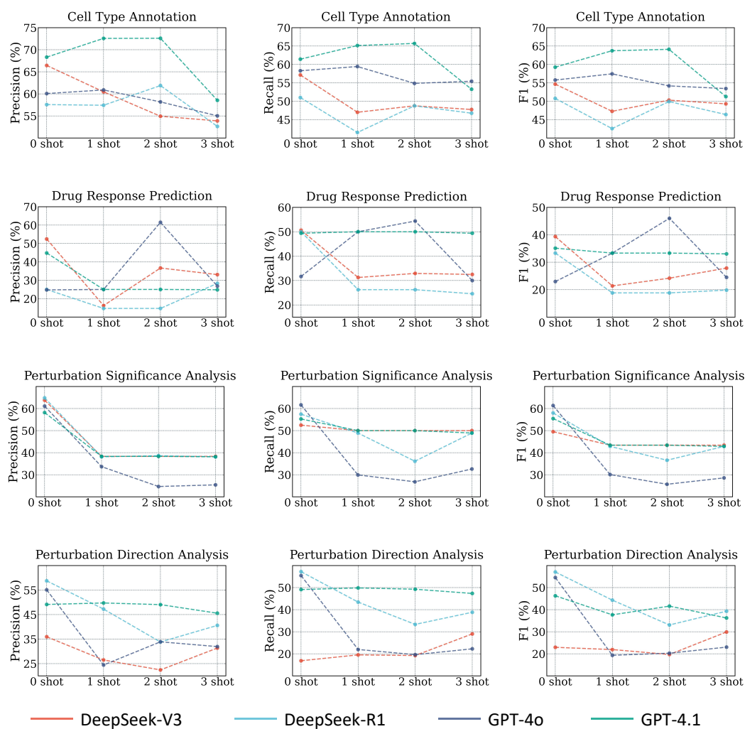
Figure 13: Precision, Recall, and F1 score comparison under few-shot settings.
