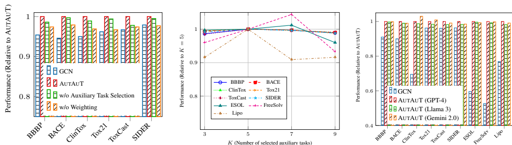
(a) Relative performance comparison of AUAUT w/ and w/o task selection and adaptive weighting. (b) Relative performance across datasets for K \in \{3, 5, 7, 9\} on the Graphormer with AUAUT. (c) Relative performance comparison of AUAUT and AUAUT variants with different LLMs.
