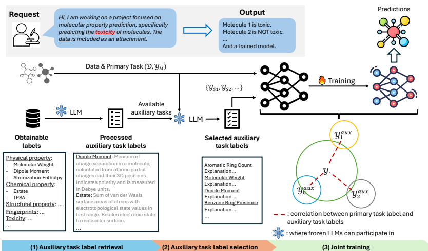
Figure 1: Overview of the AUTAUT framework. There are three main steps: (i) Auxiliary task retrieval : AUTAUT leverages the information retrieval capabilities of LLMs to retrieve a diverse set of obtainable auxiliary tasks from online resources or domain-specific databases. (ii) Auxiliary task selection : AUTAUT guides LLMs to evaluate the relevance of each auxiliary task to the primary task and select the most relevant ones. (iii) Joint training : AUTAUT employs a dynamic weighting strategy to adjust the contribution of each auxiliary task during training, ensuring that they provide meaningful supervision without diluting the primary task signal.
