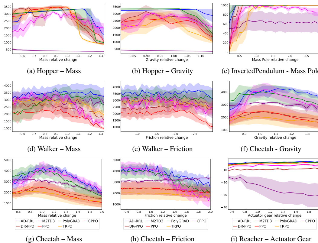
Figure 2: Average return across variations in selected physics parameters. Shaded regions indicate \pm one standard error.
