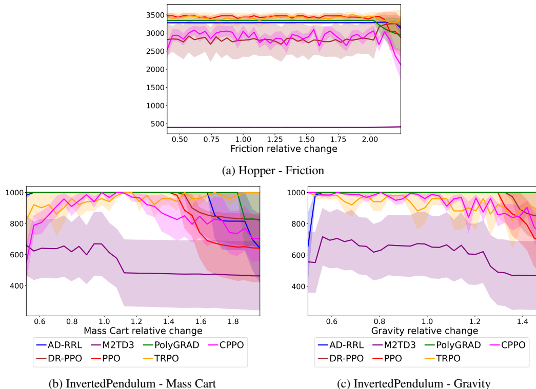
Figure 4: Average Return for varying physical parameters. Shaded areas represent one standard error over 5 runs.
