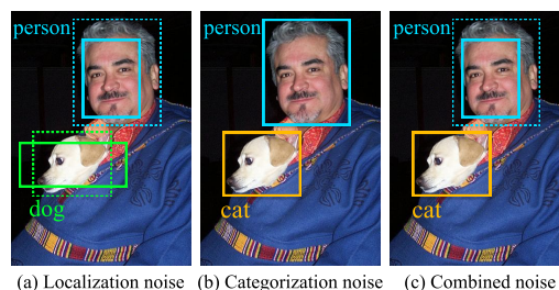
(a) Localization noise (b) Categorization noise (c) Combined noise Figure 1: Comparison of label noise types in object detection: (a) Localization only. (b) Categorization only. (c) Combined localization and categorization noise.
