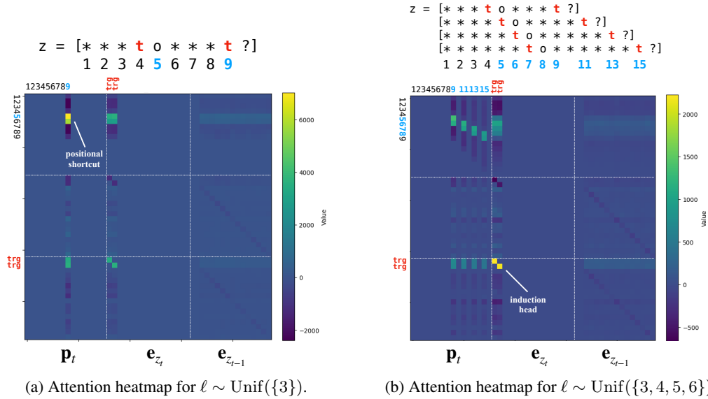
Figure 2: Attention heatmaps of \mathbf{W}^{KQ} when the pretraining sequence diversity is small (left) and large (right). In the left figure, there is a strong positional shortcut that links position 9 to position 5 (the correct position in pretraining data), whereas in the right figure, the trigger positions are more dispersed, weakening this shortcut. Instead, a signal corresponding to induction head – detecting tokens after trigger – becomes dominant.
