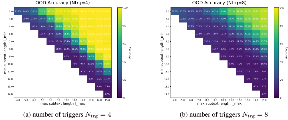
Figure 3: Out-of-distribution accuracy map over varying \ell_{\min} (vertical) and \ell_{\max} (horizontal); moving right indicates greater diversity of \ell in the pretraining distribution.
