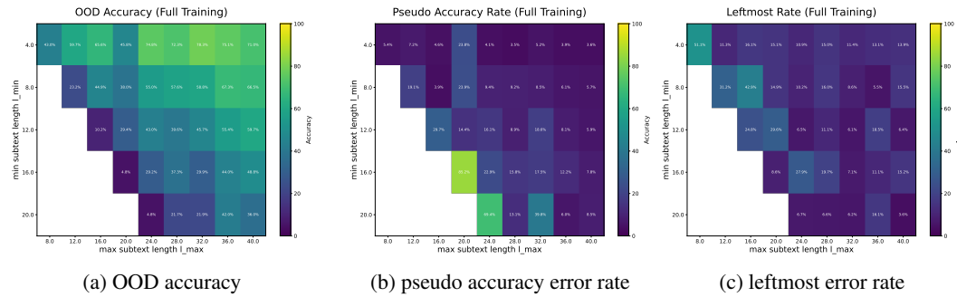
Figure 4: Accuracy map over \ell_{\min} (vertical), \ell_{\max} (horizontal) for a 3-layer transformer trained with AdamW.
