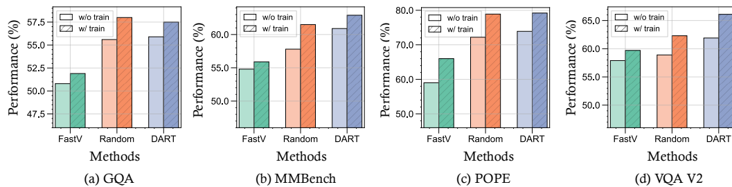
Figure 6: Following model architecture and training data of LLaVA-v1.5-7B, we apply the Random token compression for token consistency distillation during training. Here, “w/o train” denotes the vanilla LLaVA. During inference, all methods achieve a token compression ratio of 88.9%.
