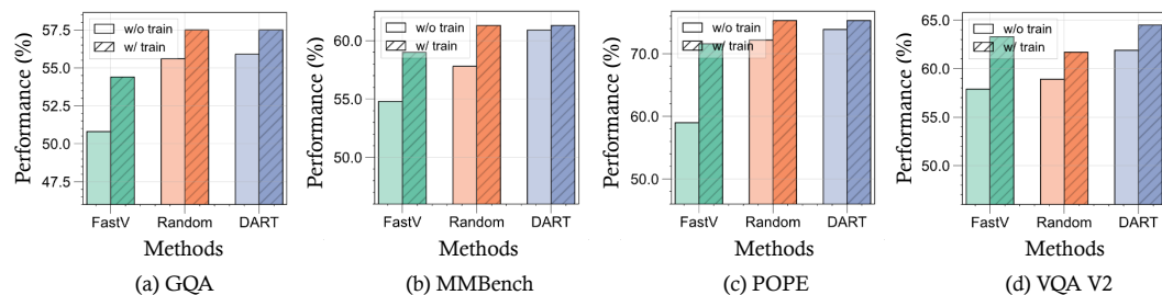
Figure 7: Following model architecture and training data of LLaVA-v1.5-7B, we apply the FastV for token consistency distillation during training. Here, “w/o train” denotes the vanilla LLaVA. During inference, all methods achieve a token compression ratio of 88.9%.
