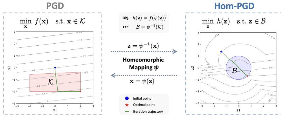
Figure 1: Hom-PGD Framework: Hom-PGD conducts the standard PGD algorithm in the transformed space by a homeomorphic mapping \psi(\cdot) , where the transformed constraint set \mathcal{B} is a simple unit ball, and the transformed objective function h(\cdot) is non-convex but structured.
