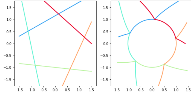
Figure 7: Illustration of the action of homeomorphism on a polyhedron. The left figure is the polyhedral constraints of problem P . Each color of line represents a constraint inequality \{\mathbf{a}_i^\top \mathbf{x} \leq b_i\} for some i . Under the homeomorphic mapping \psi , the constrained set is transformed to a ball (right figure). Each constraint inequality \{G_i(\mathbf{z}) \leq 0\} (colored differently) is non-convex in general.
