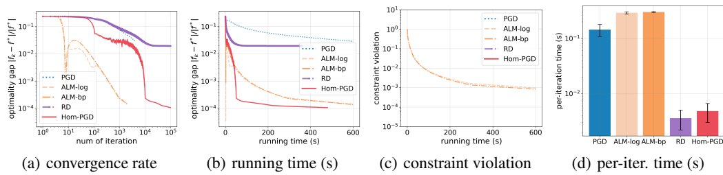
Figure 17: Convergence performance over SDP with n = 30^2 .
