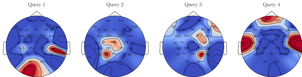
Figure 4: Visualization of the attention patterns of queries in LUNA-Base on Siena [10] topology.
