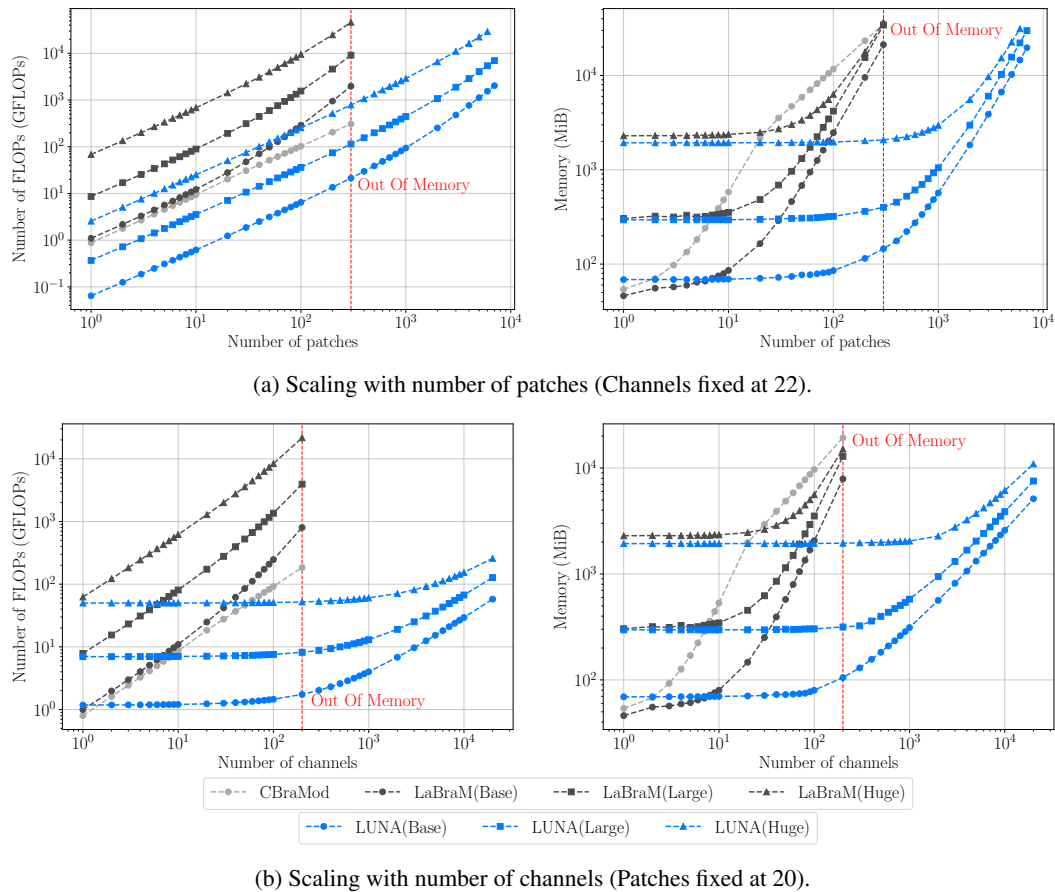
Figure 2: Computational cost scaling of LUNA and baseline models. (a) FLOPs and Memory usage vs. number of patches. (b) FLOPs and Memory usage vs. number of channels. LUNA demonstrates significantly better efficiency and scalability, especially compared to full attention (LaBraM), and favorable scaling compared to alternating attention (CBraMod) due to the fixed latent query space. CBraMod has a variable sized decoder based on the number of patches and channels; therefore, its model size as well as its resource usage grows rapidly. FLOPs are measured with fucore's FlopCountAnalysis over 50 random inputs, including encoder+decoder, with window length T , patch size P , and reported as GFLOPs per forward pass.
