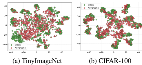
Figure 3: t-SNE visualization of clean vs. adversarial samples.
