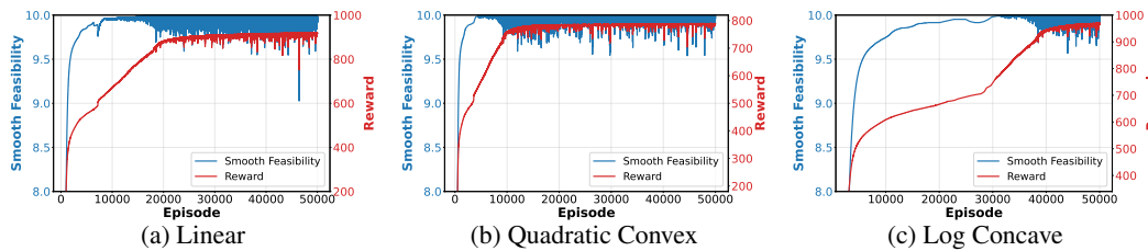
Figure 18: Evolution of Feasible Solution quality (blue, left axis) and Agent Reward (red, right axis) over training episodes.
