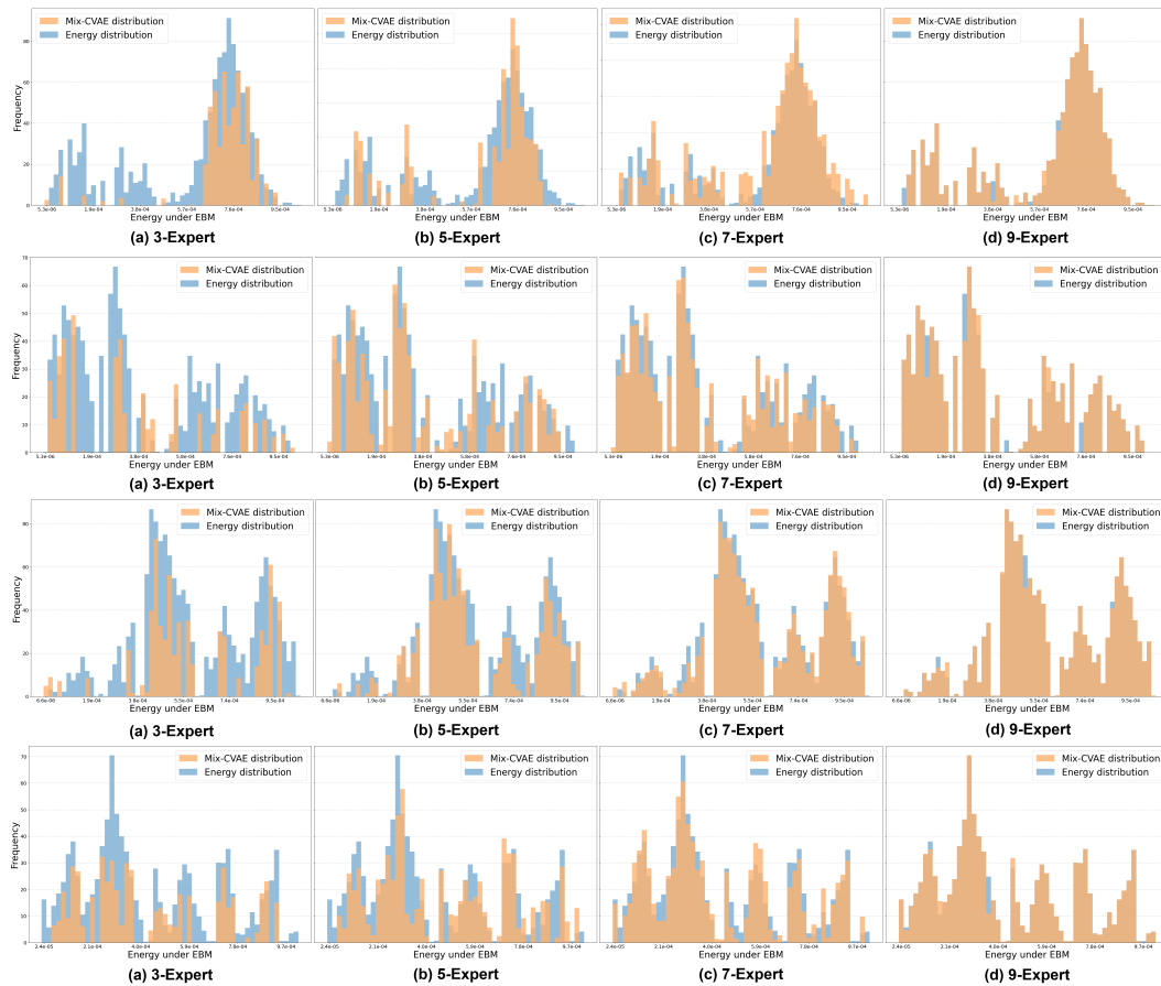
Figure 13: Impact of adding experts on real-world networks . From top to bottom: results on Email, Gnutella, RoadCA, and Skitter networks.
