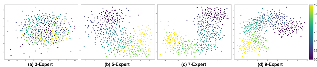
Figure 14: An example of conditional latent space visualization for the trained Mix-CVAE on the same synthetic graph and pairs but different thresholds. Points represent latent vectors \mathbf{z} , colored by threshold T . Clear clustering shows the latent space captures meaningful patterns.
