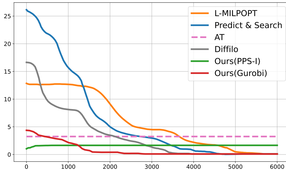
Figure 19: Convergence comparison of the relative optimal gap across Hephaestus and baseline methods under the Linear cost setting. The relative optimal gap measures the percentage deviation from the best-known (optimal) solution, with lower values indicating better performance. Existing ML-based methods (L-MILPOPT, Predict-and-Search, DiffILO) gradually reduce their gaps over time through external solver refinement (e.g., Gurobi), but typically require thousands of seconds. In contrast, Hephaestus with Gurobi (red curve) rapidly converges to zero gap due to its high-quality initial solutions and efficient generative modeling. Hephaestus with PPS-I (green curve), although not exact, achieves low gaps in significantly less time, offering a fast and practical alternative.
