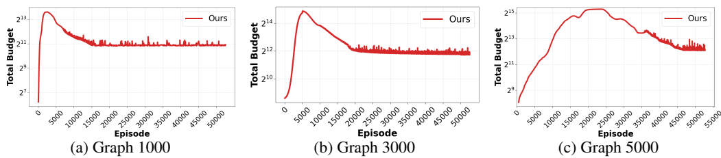
Figure 16: Evolution of Total Budget during the Refine phase (RL agent training)
