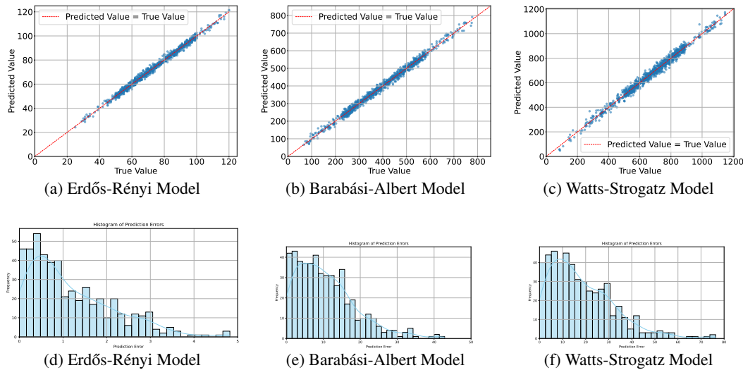
Figure 7: Predictive Accuracy Across Different Graph Topologies.
