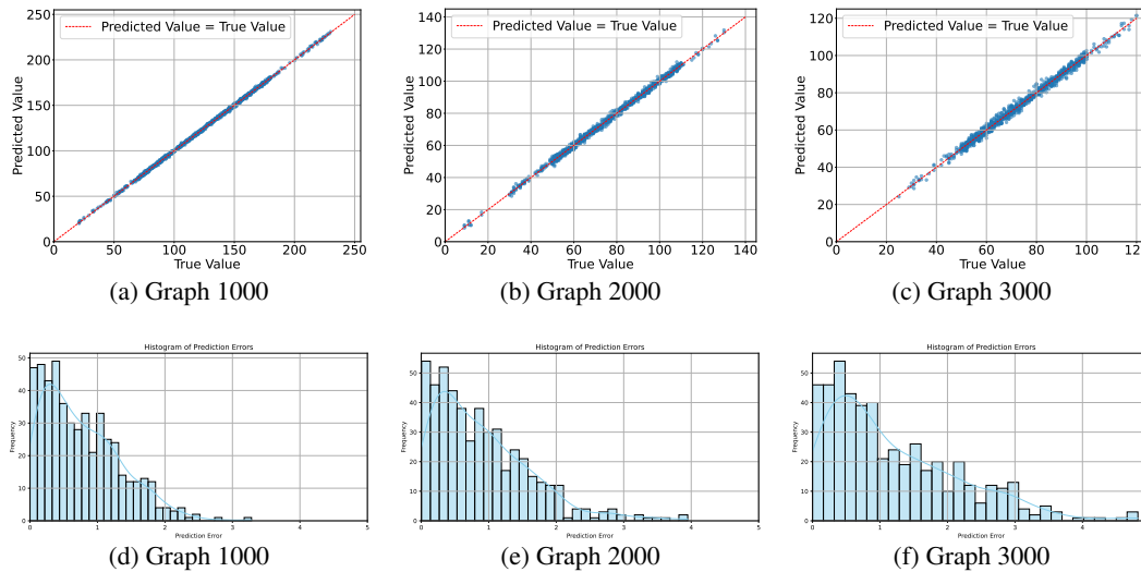
Figure 6: Predictive Accuracy Across Different Graph Sizes.
