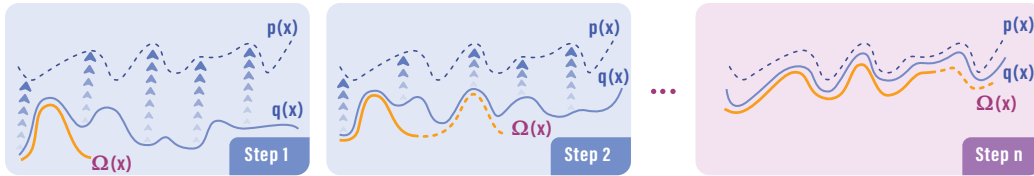
Figure 2: At each iteration, the generative model \Omega(x) adds an expert in regions where the log-ratio \chi(x) = \log(q(x)/\Omega(x)) exceeds \delta , thereby covering more of q(x) . Meanwhile, q(x) adapts to align with p(x) . As the steps progress, q(x) increasingly approximates p(x) , and \Omega(x) , augmented by new experts, converges to q(x) , ultimately yielding p(x) \approx q(x) \approx \Omega(x) .
