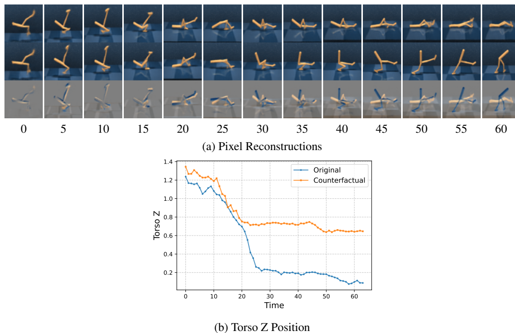
Figure 6: (a) (Pixel Modality) Counterfactual Trajectories in Pixel Space : Top: Original imagined trajectory of the Walker Walk under default gravity and actuator strength. Middle: Perturbed trajectory after adding noise \Delta to the top-ranked latent dimension \mathbf{z}_3 . Original trajectory shows the Walker failing to recover after a fall. The perturbed trajectory with enhanced actuator strength enables recovery and forward locomotion. Bottom: Pixel-wise differences ( \delta = |\hat{o}_t - \hat{o}'_t| ). The counterfactual agent refines leg kinematics (frames 30-45) and stabilizes upright (frames 50-64). (b) (Featurized Modality) Torso Z-Position Under Latent Perturbation : Comparison of original (blue) and counterfactual (orange) torso heights. The perturbed \mathbf{z}_3 trajectory maintains higher elevation after time step 20, reflecting successful stabilization and locomotion.
