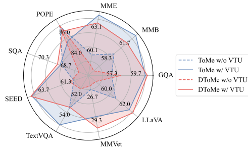
Figure 5: Importance of Virtual Token Unmerging (VTU). We ablate the performance of LLaVA 1.5 with two token reduction methods applied to the visual encoder—ToMe (fixed-length) and DToMe (dynamic-length). We observe that applying VTU significantly improves performance on 8 out of 9 benchmarks, demonstrating robustness to varied token reduction methods.
