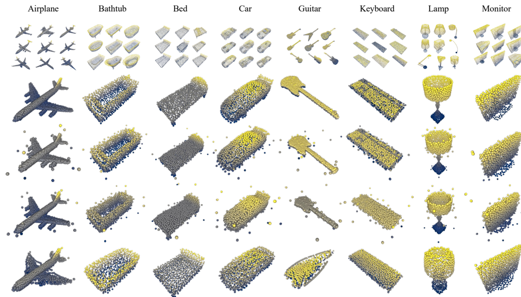
Figure 3: Comparison of synthetic datasets distilled from the ModelNet40 [25] dataset. Point clouds were colorized according to the y-coordinates. From top to bottom, the original dataset (first), initialized point cloud models (second), and the distilled synthetic datasets by using DC [30] (third), DM [29] (fourth), and the proposed method (fifth).
