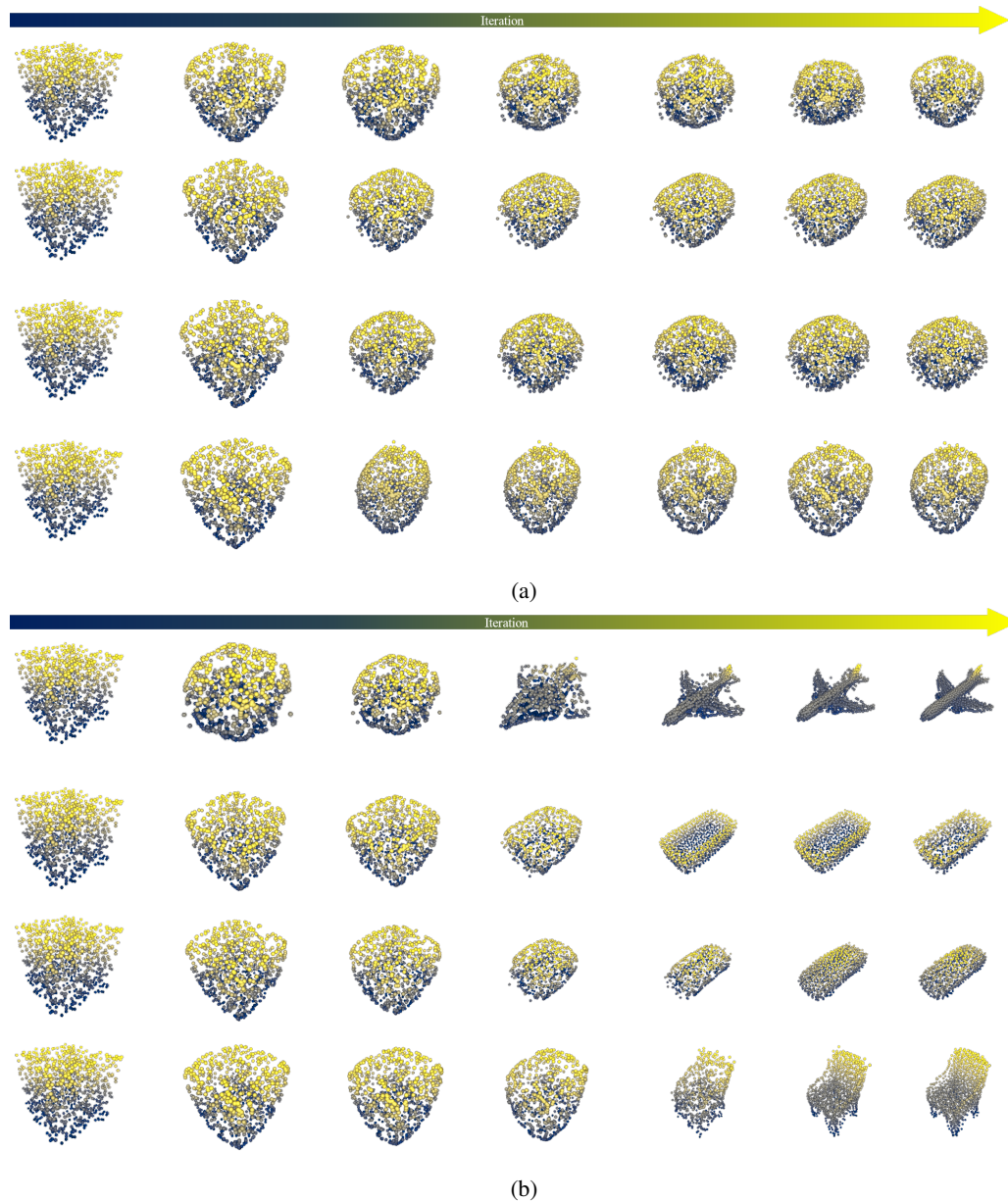
Figure 9: Optimization process in the ModelNet40 at PPC 1 initialized from uniform noise, distilled by using (a) DM [29] and (b) the proposed method.
