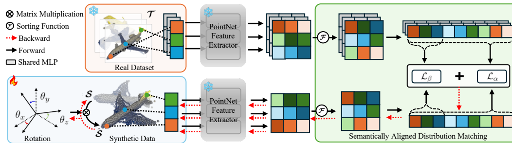
Figure 1: The overall framework of the proposed dataset distillation method for 3D point clouds.
