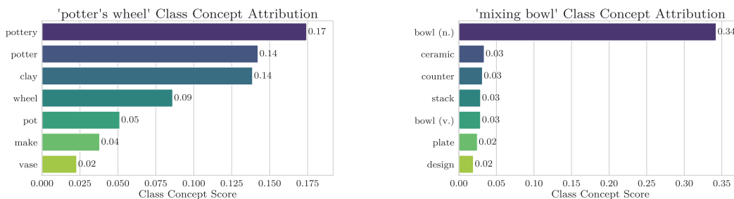
Figure 6: Average class concept scores for ImageNet classes “potter’s wheel” and “mixing bowl”.
