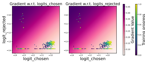
Figure 2: SimPO
