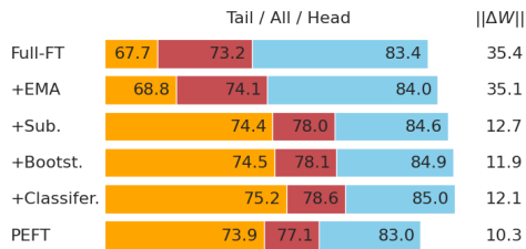
Figure 5: Performance and weight change comparison across different stages of LT-Soups.
