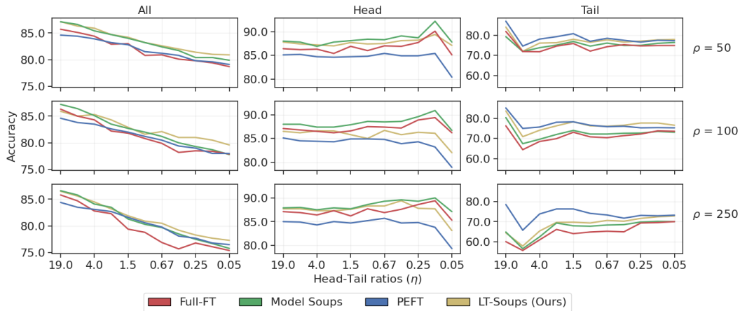
Figure 1: Performance of baselines and LT-Soups on the CIFAR100 benchmark varying \rho and \eta . While full fine-tuning generally outperforms PEFT on head classes, PEFT demonstrates superior performance on tail classes. In contrast, our approach maintains robust accuracy across all imbalance settings, showing resilience to shifts in both the sample distribution and class structure.
