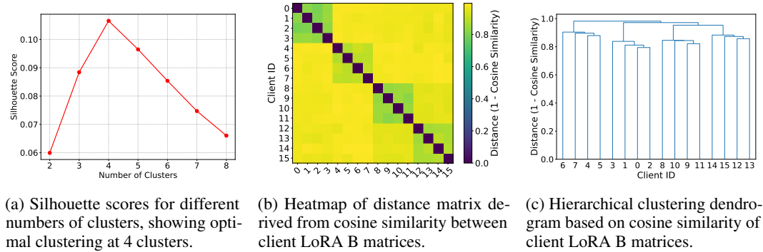
Figure 7: Visualization of client clustering results based on cosine similarity of LoRA B matrices.
