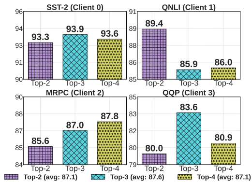
Figure 4: Comparison on accuracy of clients using different top- k strategies under the task-heterogeneous setting.
