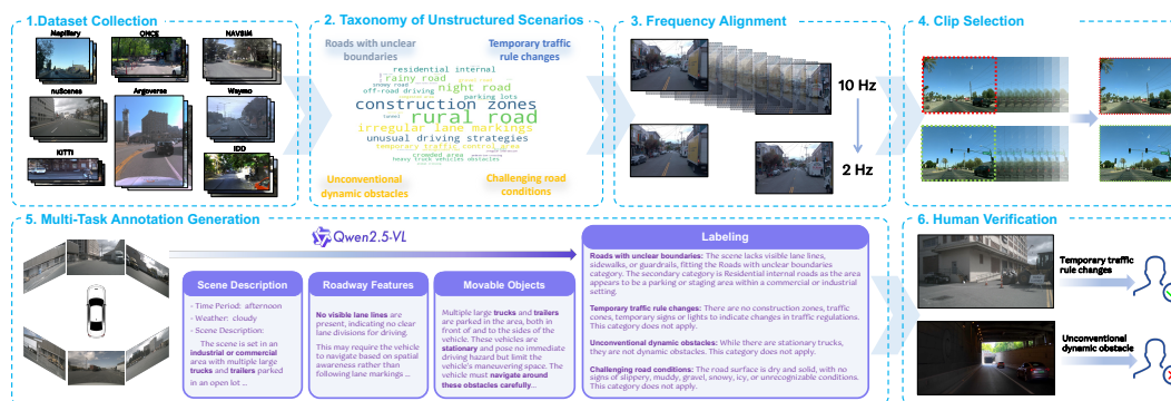
Figure 3: Data Processing and Annotation Pipeline for the Impromptu VLA Dataset. The diagram outlines the sequential process for creating our dataset, starting from raw data collection and scenario taxonomy definition (Sec. 2.2, through frequency alignment and keyclip selection, to multi-task annotation generation via Qwen2.5-VL (including scene description, object/feature analysis, and labeling), and concluding with rigorous human verification (Sec. 2.3).
