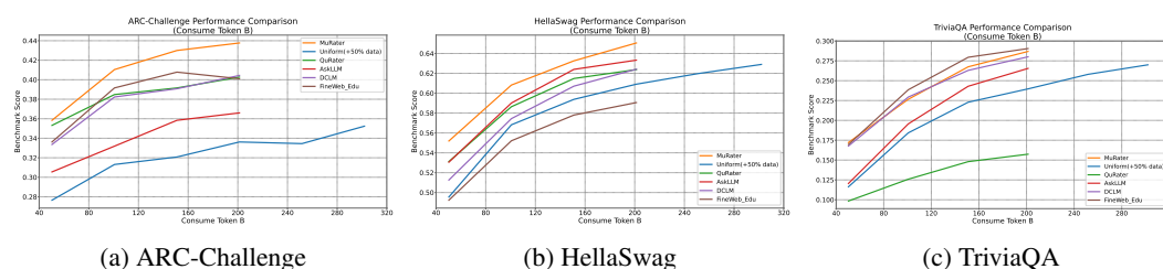
Figure 3: Performance of different selection methods on ARC-Challenge, HellaSwag, TriviaQA, and the overall average across 12 tasks during training on 200B English tokens
