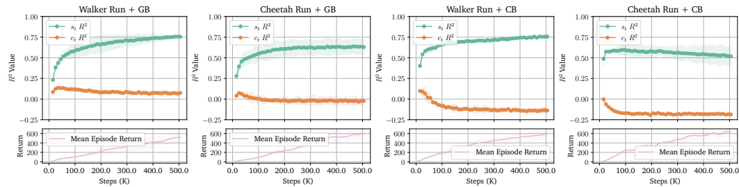
Figure 16: Coefficient of determination ( R^2 ) on DMC tasks with background distractors.
