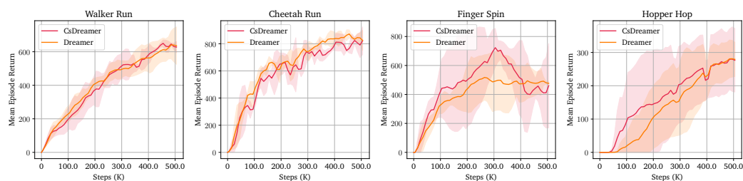
Figure 12: Performance on Standard DMC.
