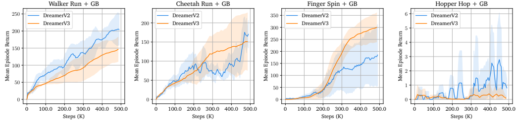
Figure 10: Performance of DreamerV2 and DreamerV3 on DMC using the gray natural videos as background.
