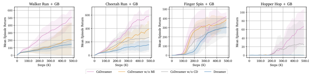
Figure 7: Ablation Performance on DMC using gray natural videos as background.
