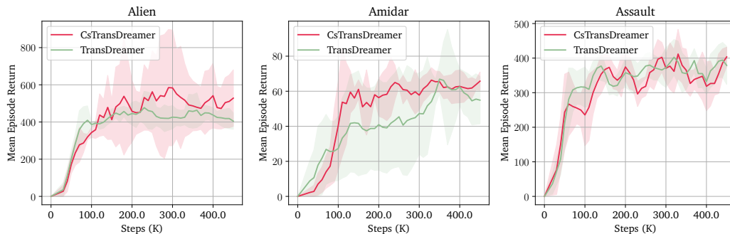
Figure 17: Transformer-based results on three Atari environments.
