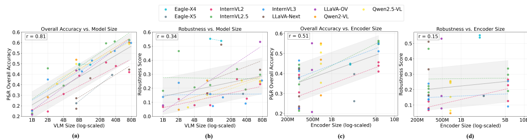
Figure 6: Correlation analysis between performance and size across MLLM families: (a) Overall accuracy vs. model size ( r = 0.81 ), (b) Robustness vs. model size ( r = 0.34 ), (c) Overall accuracy vs. encoder size ( r = 0.51 ), (d) Robustness vs. encoder size ( r = 0.15 ). Total model scaling strongly impacts perspective understanding, while vision encoder size has a limited influence on robustness.
